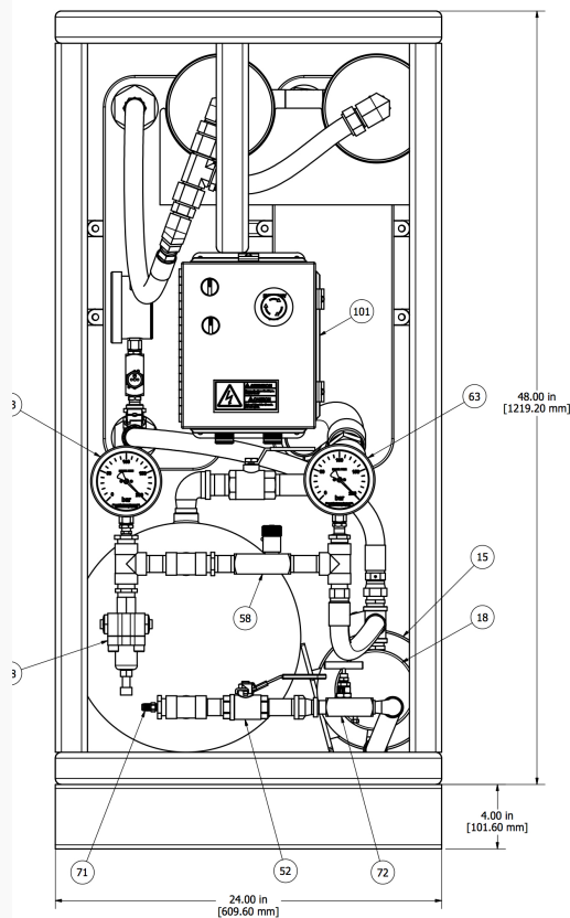
RIGHT VIEW
