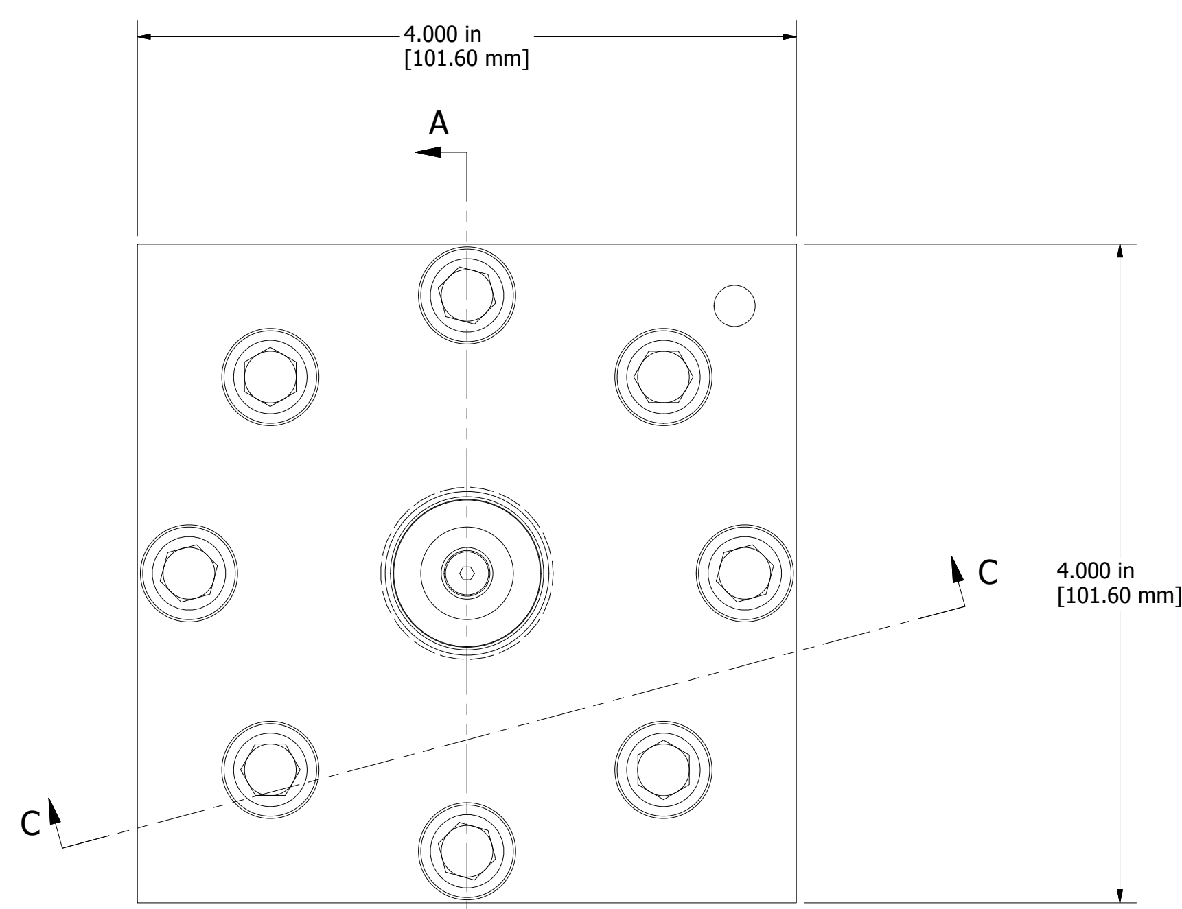
FRONT VIEW SCALE 1.25
