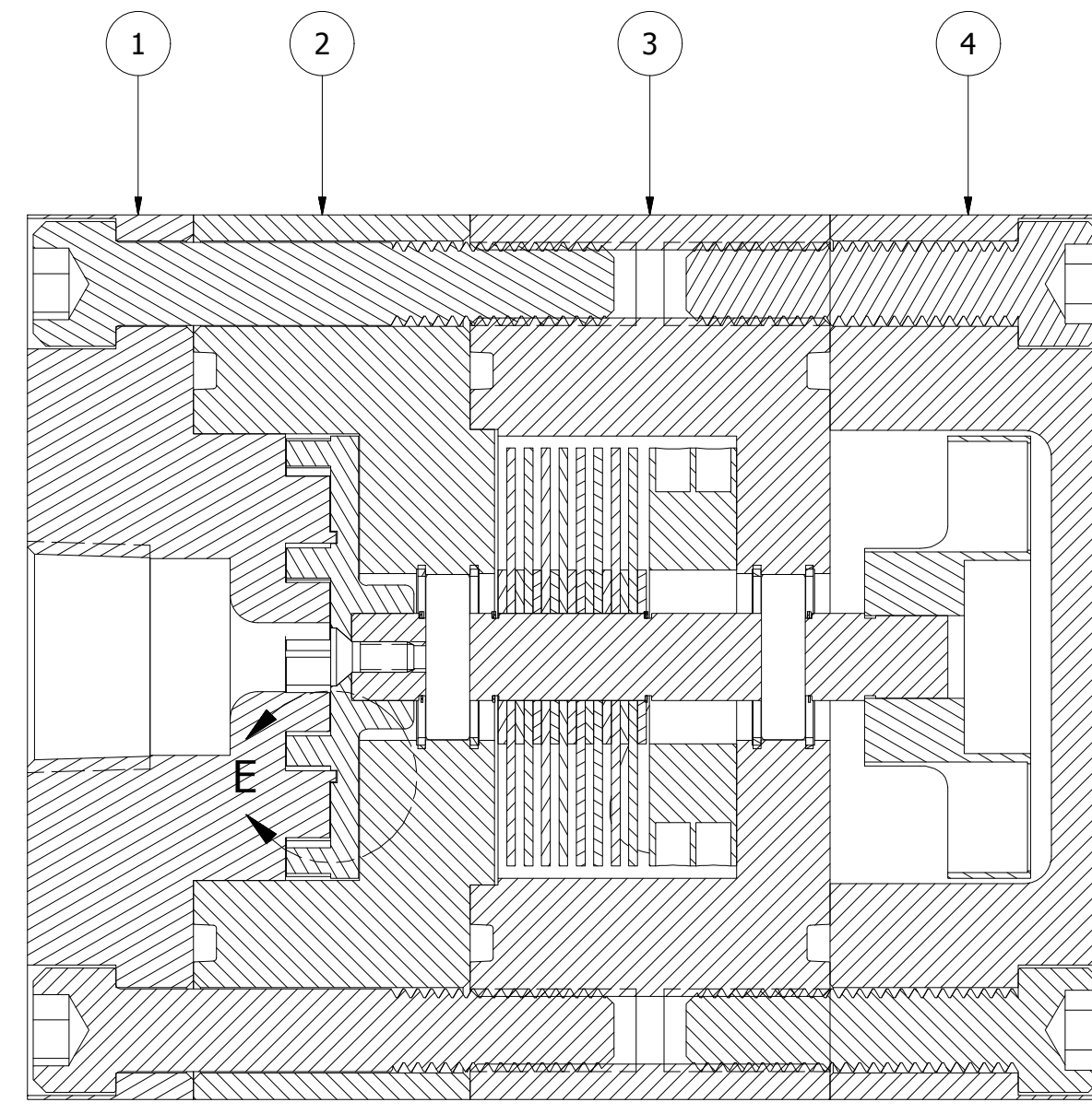
SECTION D-D SCALE 1.25
