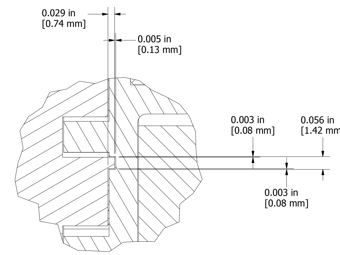
DETAIL E - Labyrinth Seal SCALE 4 : 1
