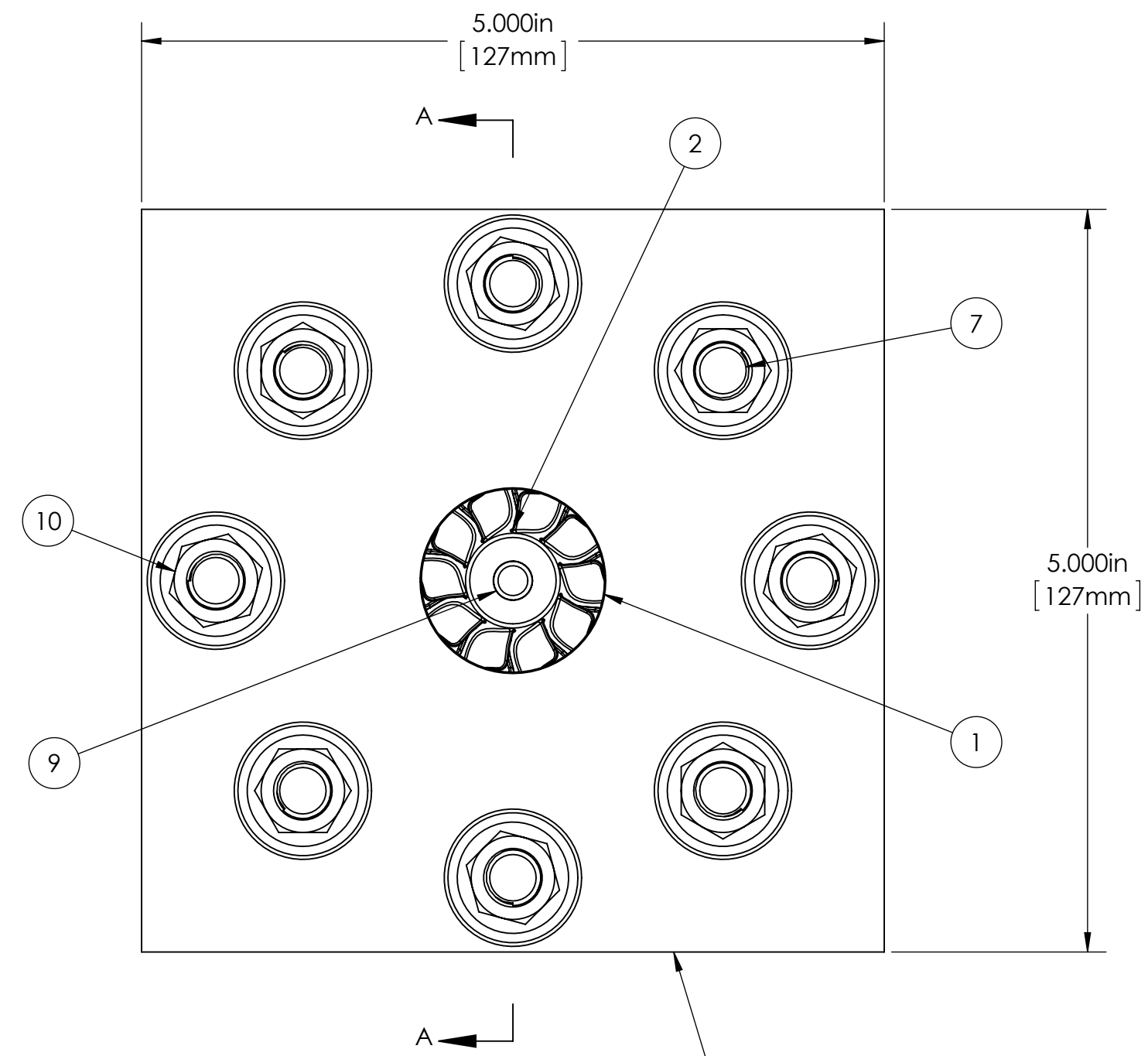
FRONT VIEW SCALE 1:1
