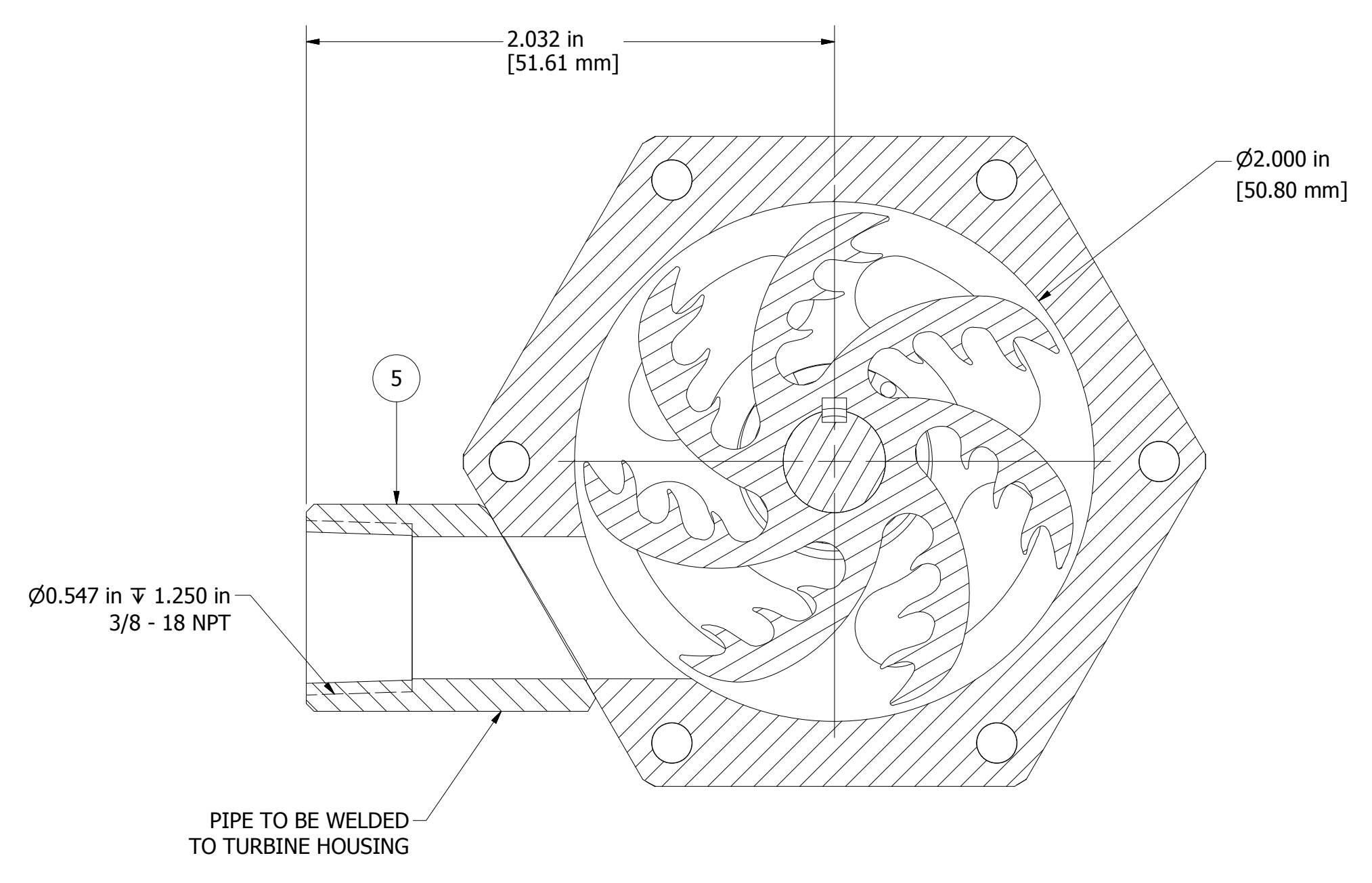
SECTION C-C SCALE 2 : 1
