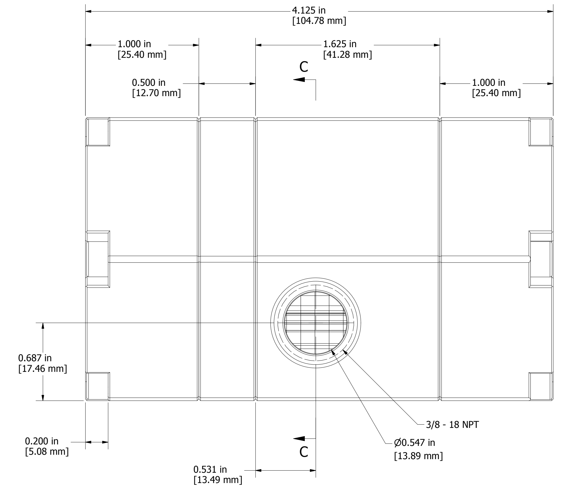
SIDE VIEW SCALE 2 : 1
