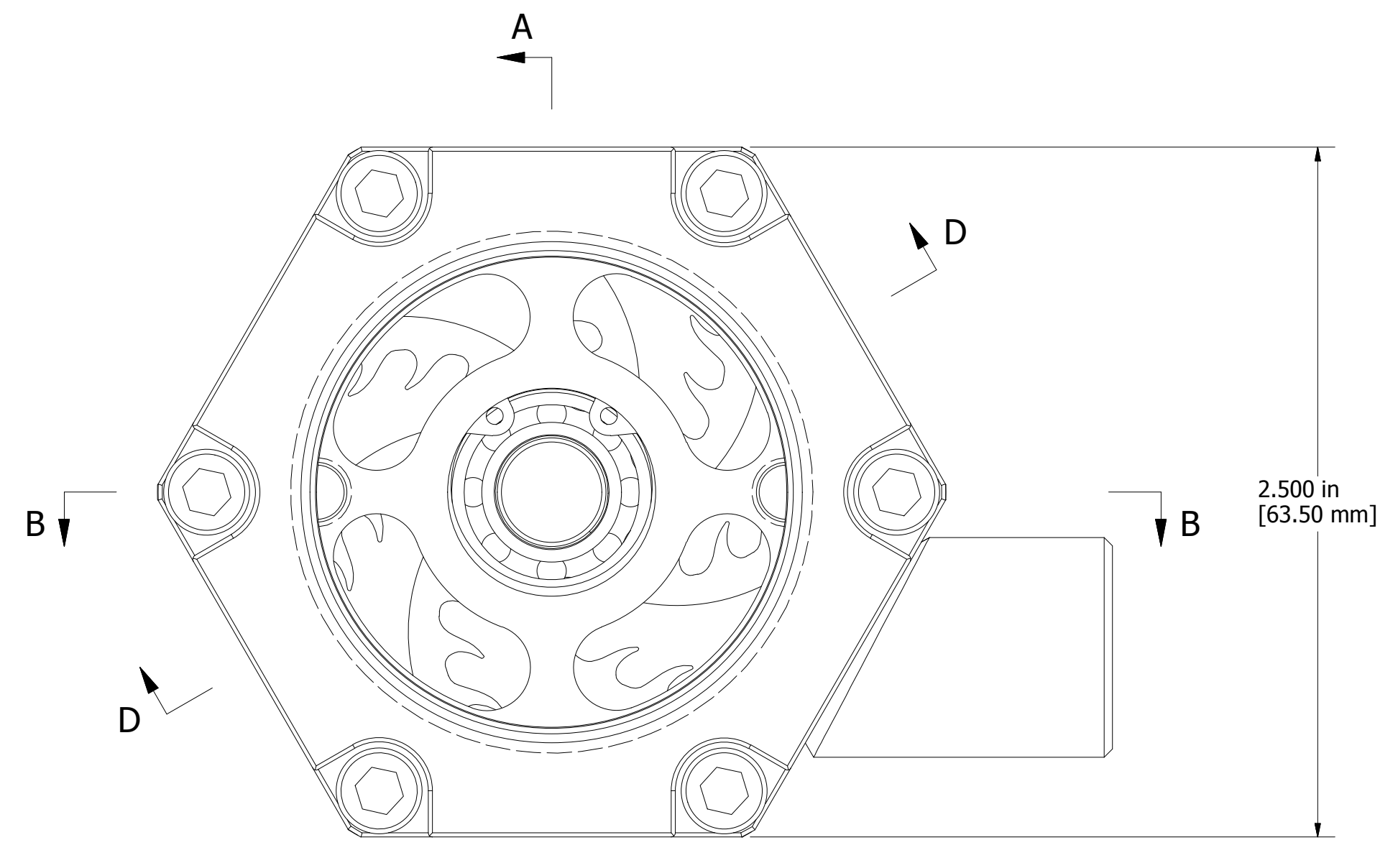
FRONT VIEW SCALE 2 : 1
