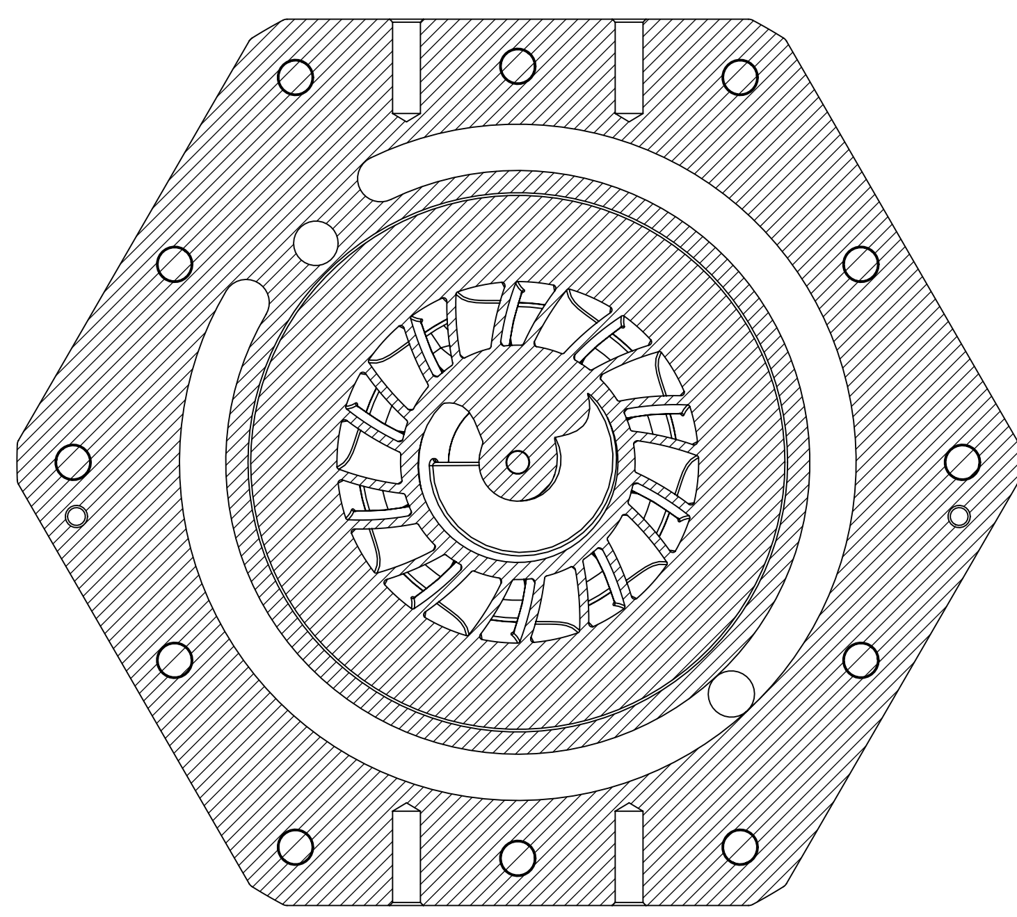
SECTION C-C SCALE 1:1.5
