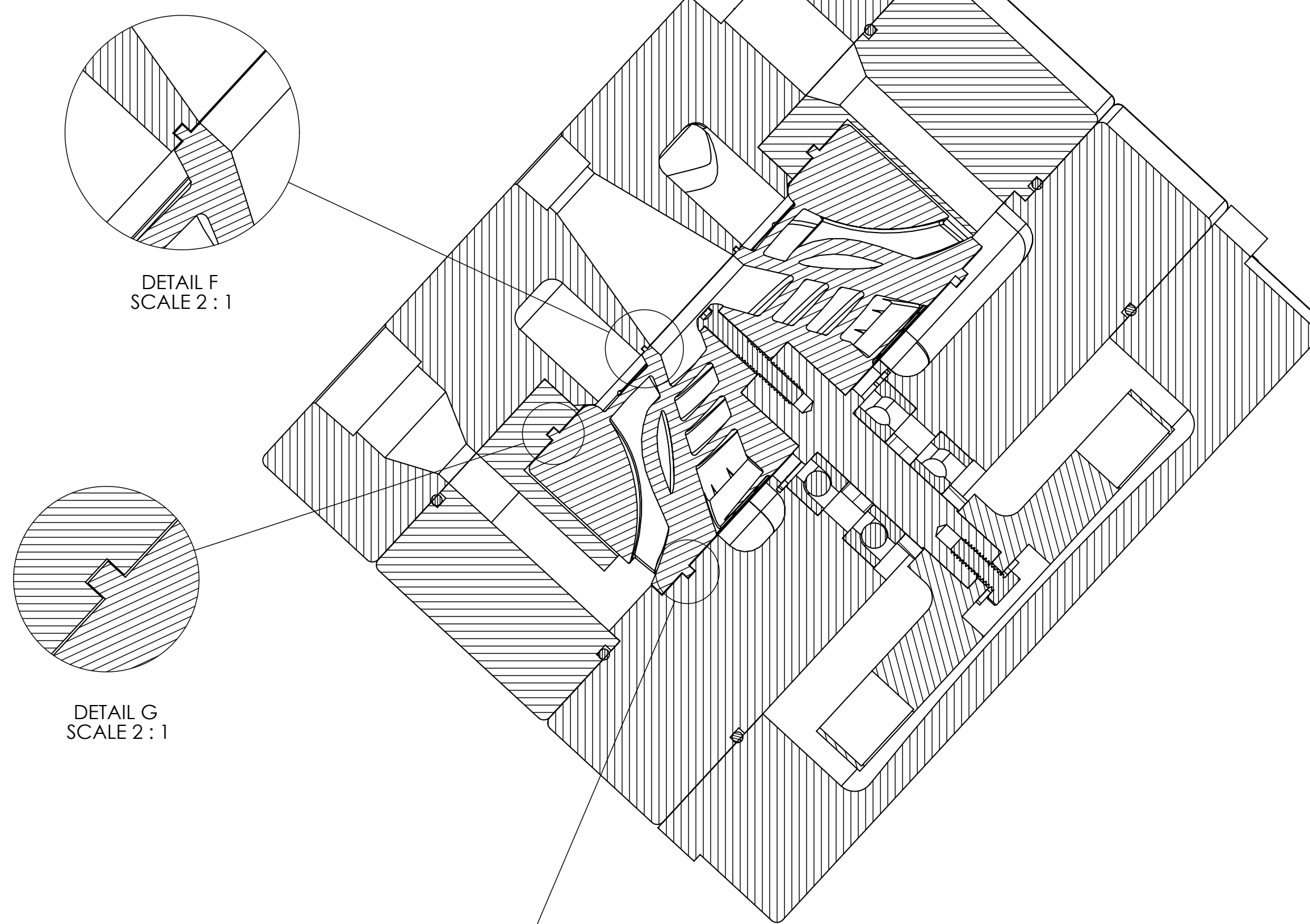
SECTION E-E SCALE 1:1.5
