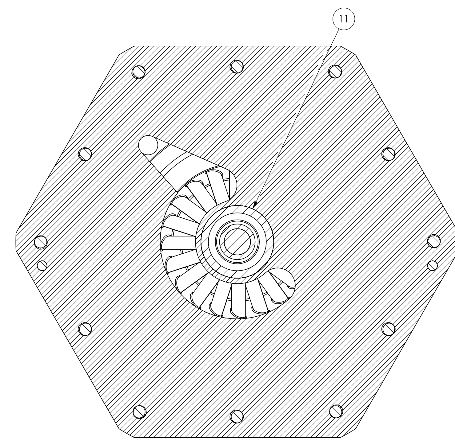
SECTION D-D SCALE 1:1.5
