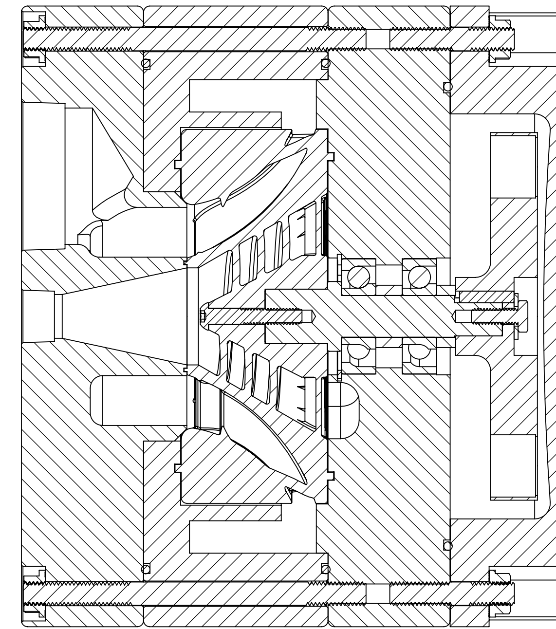
SECTION AA-AA SCALE 1:1.5
