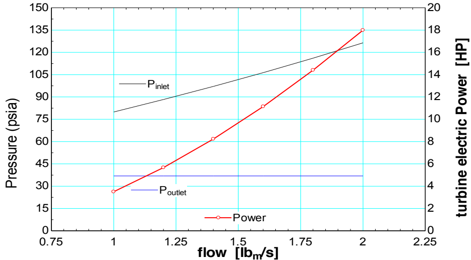
ROT15 Performance R245fa, 3050 RPM
